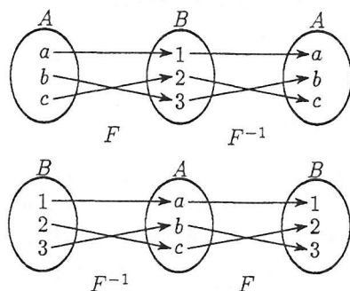
Figure 2-5: Composition of one-to-one correspondence with its inverse.
