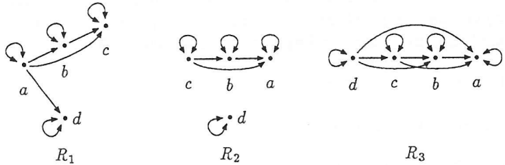
Figure 3-3: Diagrams of the weak orders in (3-21).
