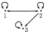
Figure 3-1: Relational diagram.
